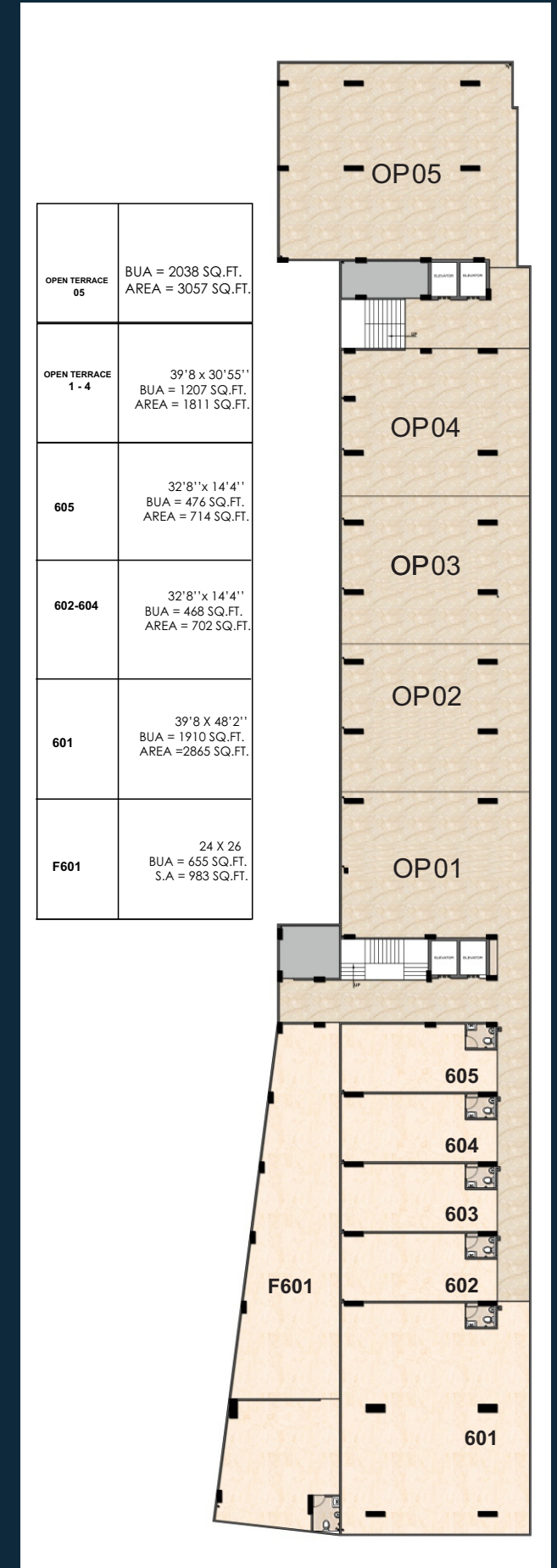
SIXTH FLOOR (TERRACE PLAN)
